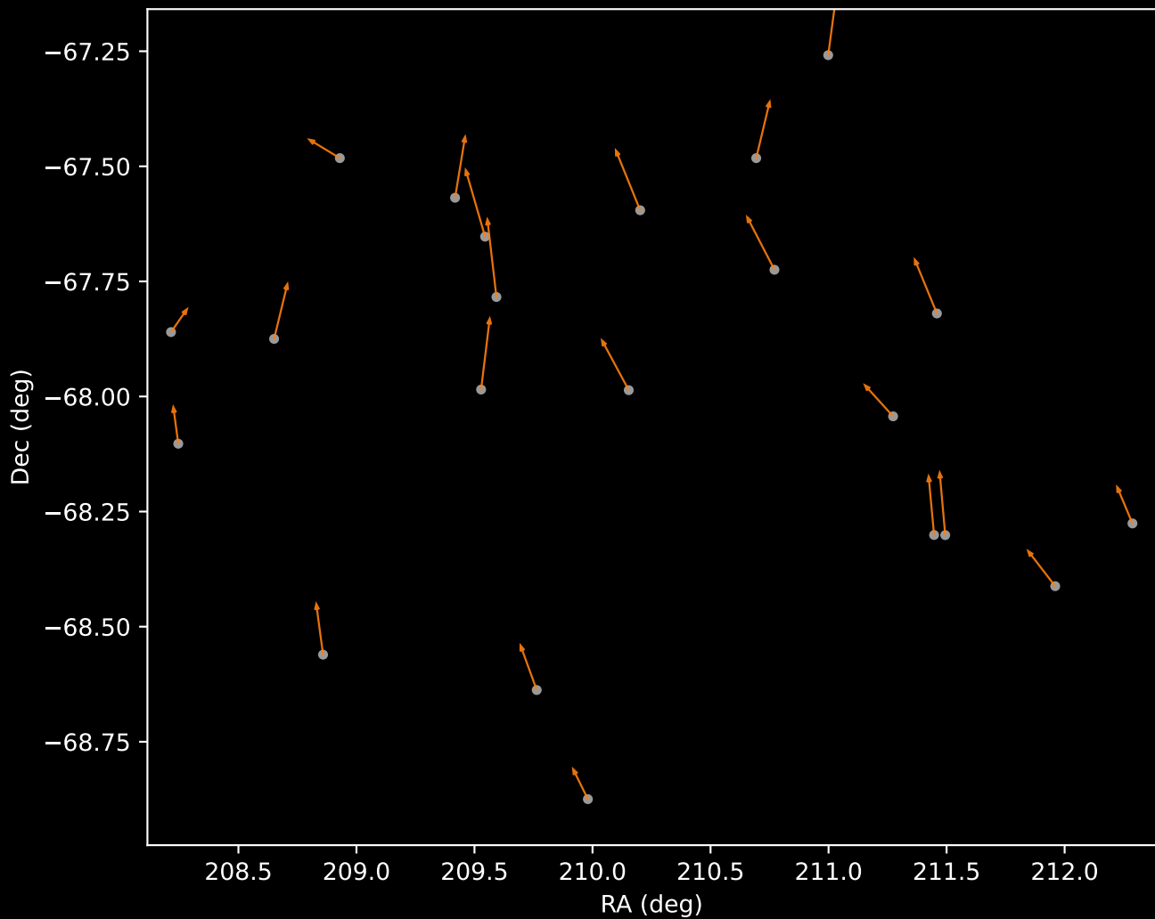
GALAH DR4 Cluster 2 Proper Motion Vectors (n=22)
