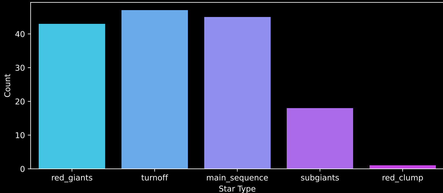
GALAH DR4 Field: [7168] Count plot of Star Type
