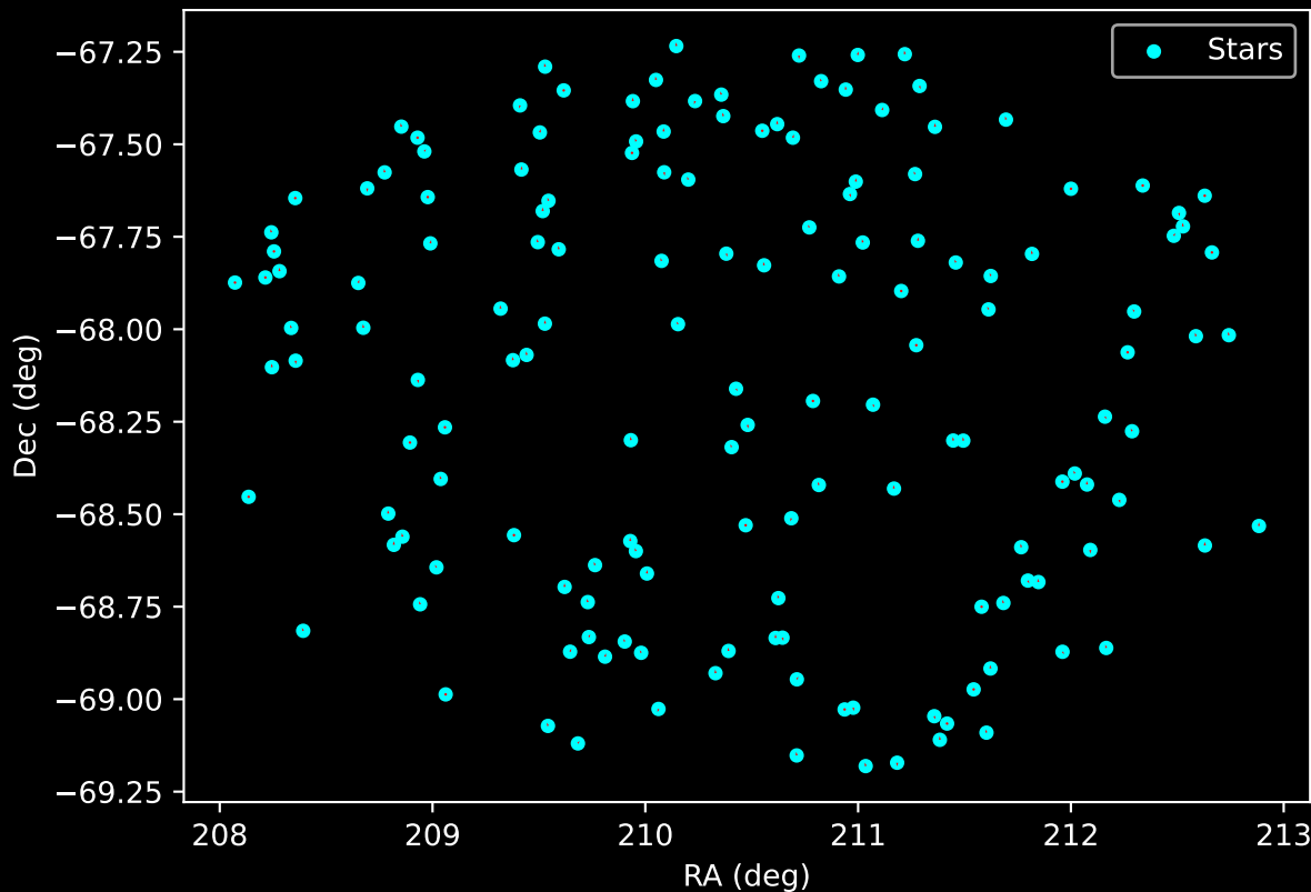
GALAH DR4 Field: [7168] Proper Motion Vectors for Gaia Star Field (n= 154)
