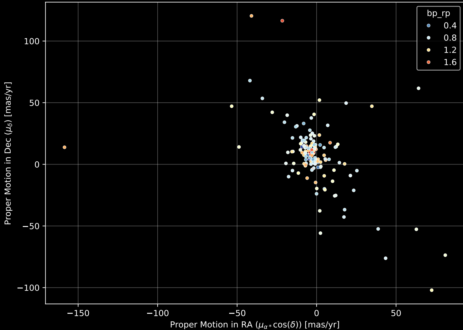
GALAH DR4 Field: [7168] Proper Motion Diagram (n= 154)
