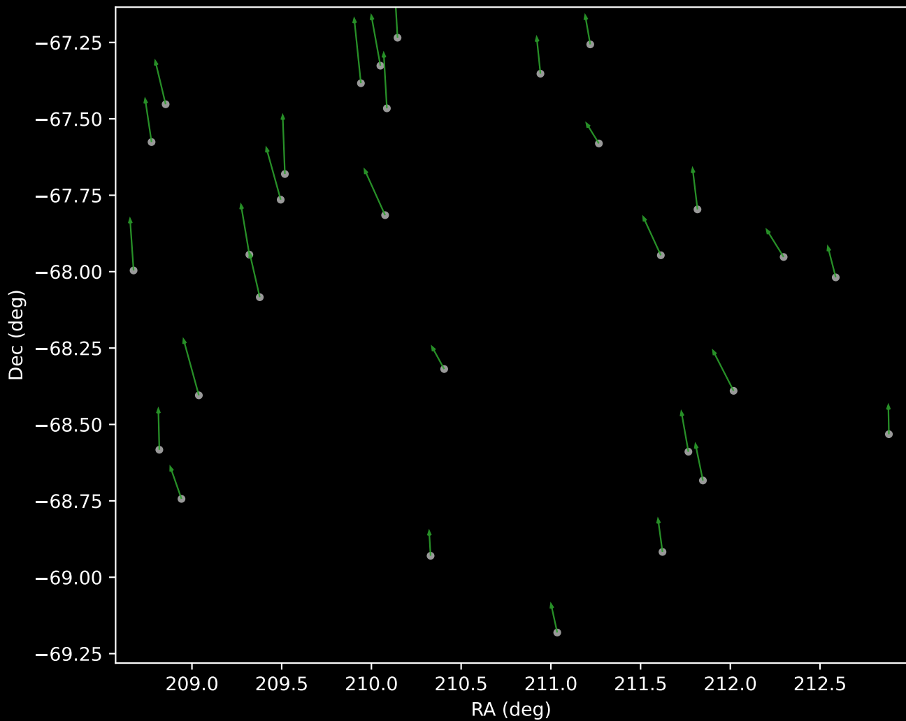
GALAH DR4 Cluster 4 Proper Motion Vectors (n=30)
