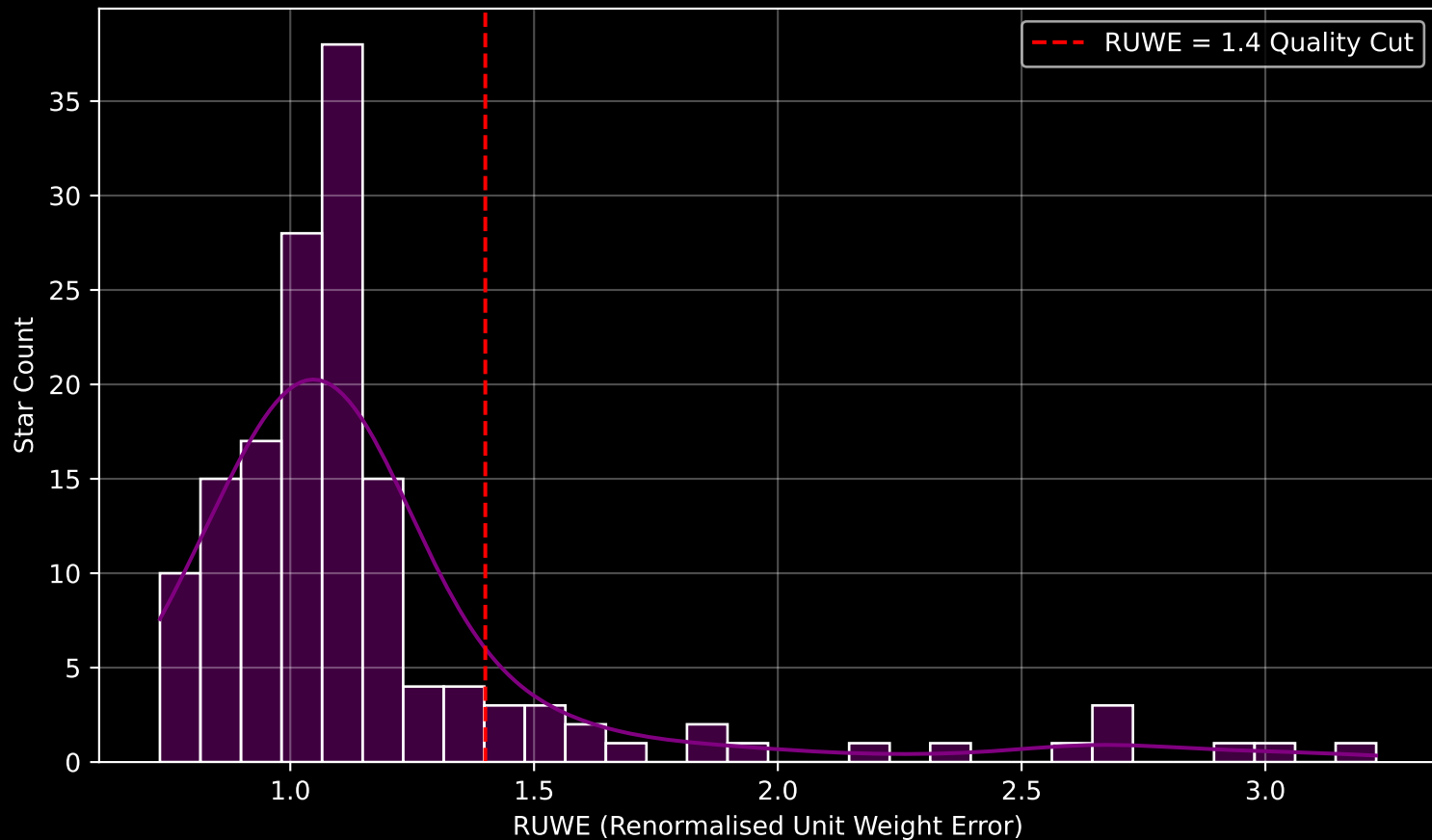
GALAH DR4 Field [7168] RUWE Distribution (n= 152)
